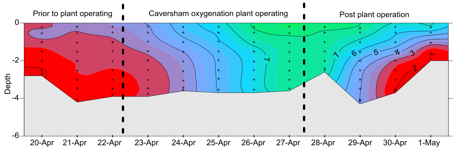
MSB: dissolved oxygen concentrations (mg/L) measured daily 3.2 km upstream of the Caversham oxygenation plant
