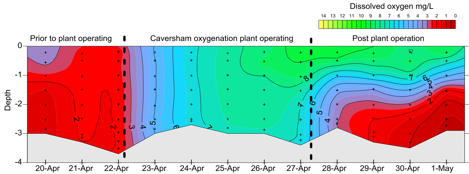
CAV: dissolved oxygen concentrations (mg/L) measured daily 0.2 km upstream of the Caversham oxygenation plant
