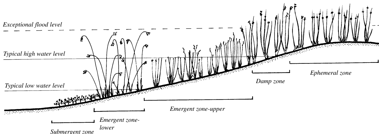
Figure 1: Wetland zones and typical distribution of some sedge and rush species.
